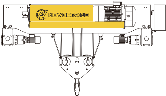
Double Girder trolley TYPE
